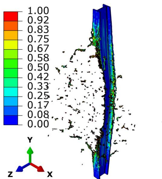
Fig. 9. Damage for M-3
