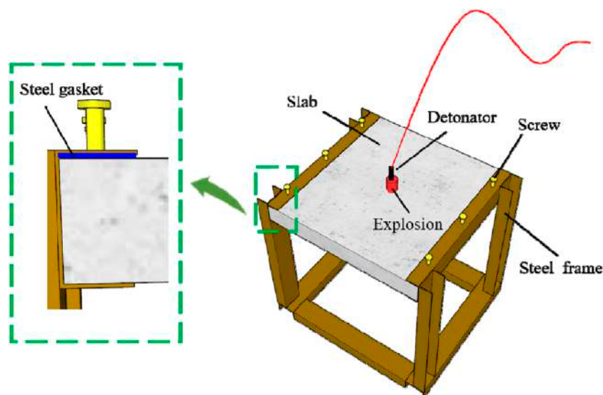
FIGURE 2 Schematic diagram of the testing device.
