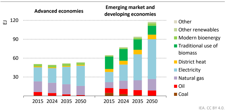
Figure 3.9 ▶ Energy demand in buildings by economic grouping and fuel in the CPS to 2050
