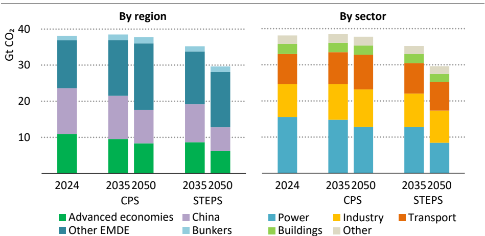
Figure 5.27 ▶ Emissions by region and sector in 2024 and by scenario, 2035 and 2050
